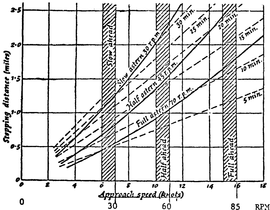
STOPPING CURVES DIAGRAM
